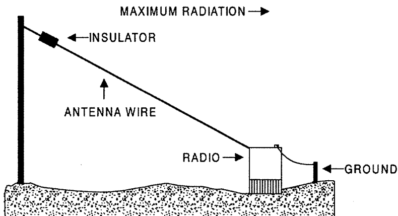
Figure 4-26. Sloping Wire.
